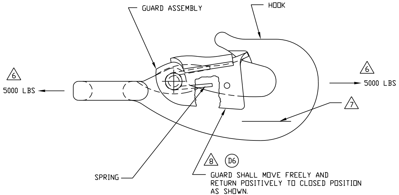
SNAP ASSEMBLY
