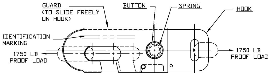
SNAP ASSEMBLY
