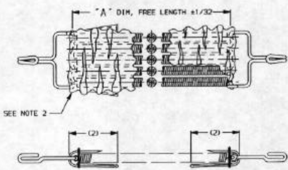
TYPICAL CONFIGURATION EXCEPT FOR -4
