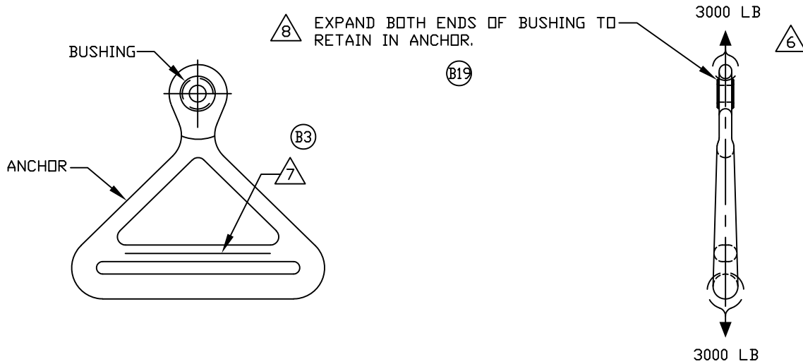
ASSEMBLY
