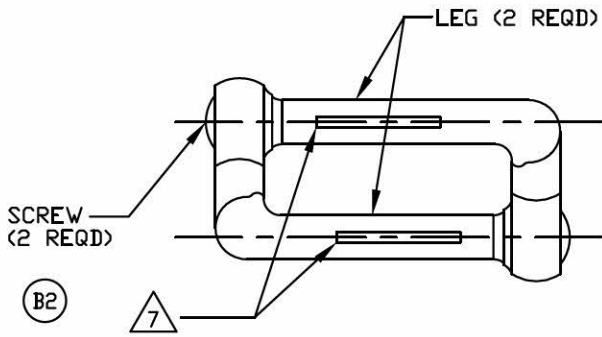
LINK ASSEMBLY -1 & -2
